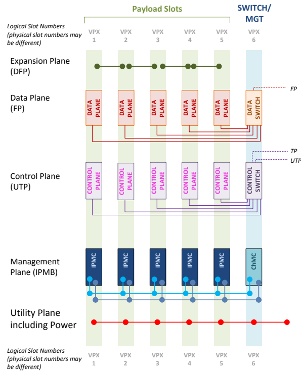
Figure 3: VTX880 Backplane Connections
