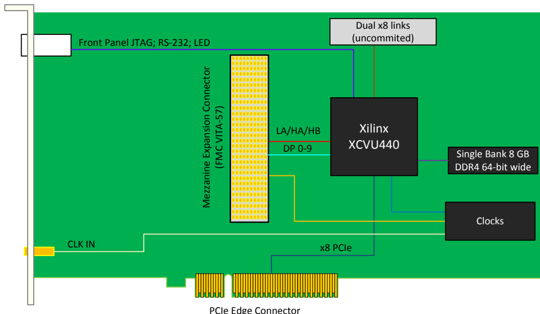
Figure 1: PCI595 Functional Block Diagram
