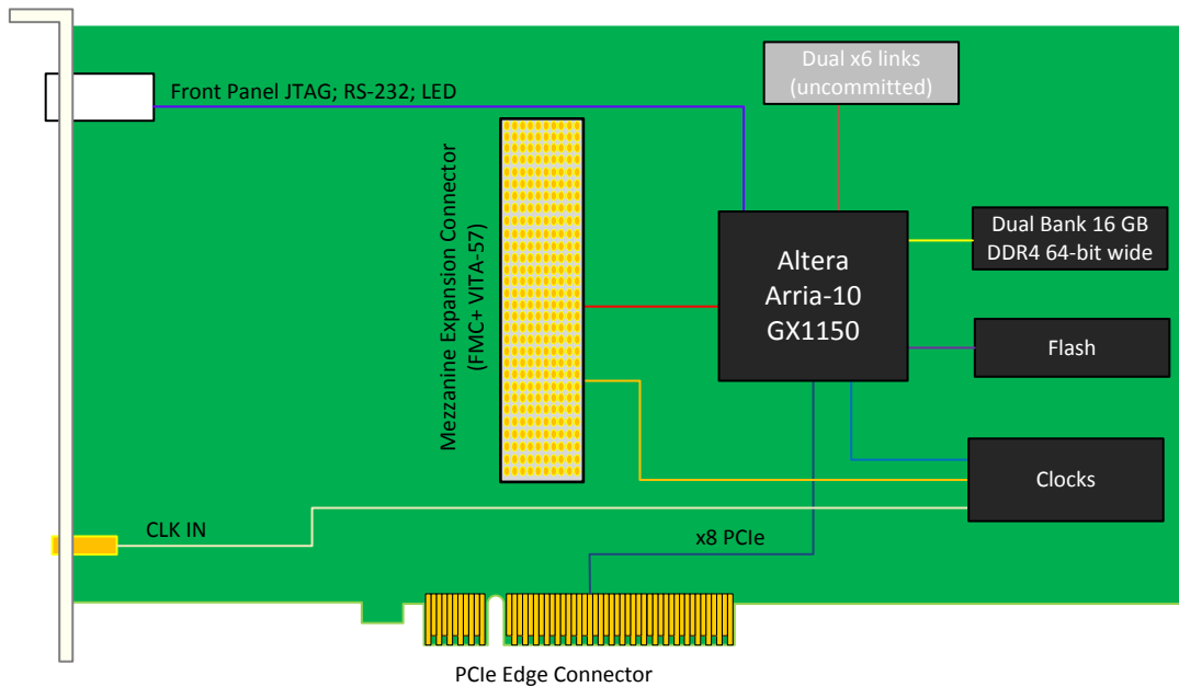
Figure 1: AMC536 Functional Block Diagram
