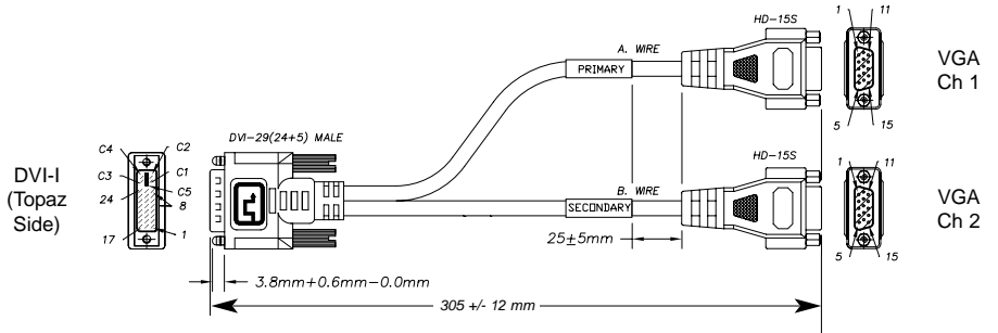
A31-00735-1011 (VSG-2/1) cable assembly
