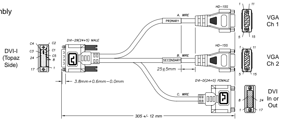
A31-00735-1012 (VSG-3/1) cable assembly
