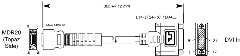
A31-00735-5012 (VLG-1/1) cable assembly
