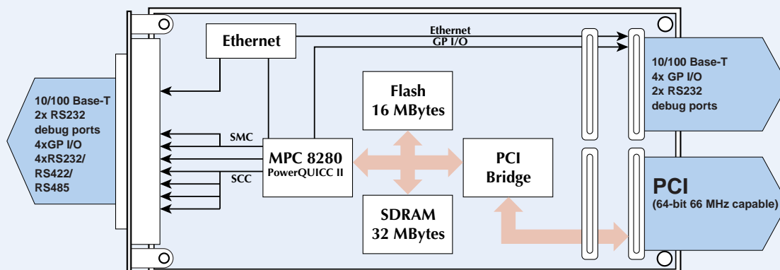
Figure 2: PrPMCQ2F Image and Functional Block Diagram
