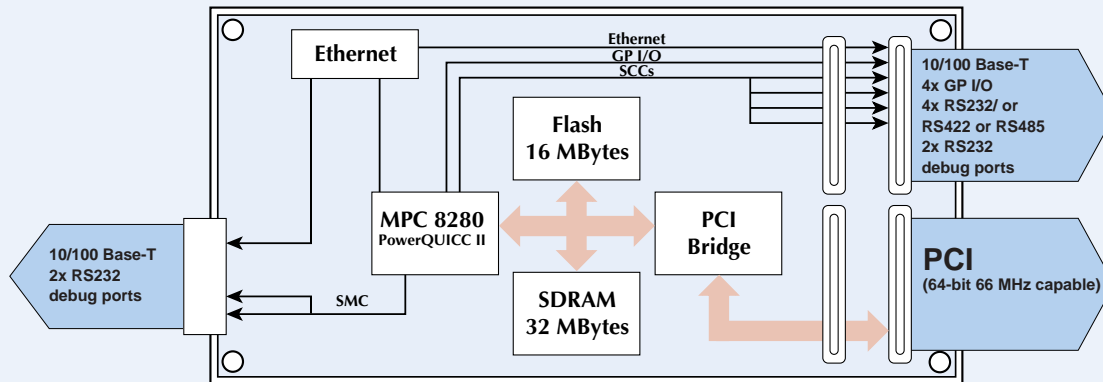
Figure 1: PrPMCQ2R Image and Functional Block Diagram
