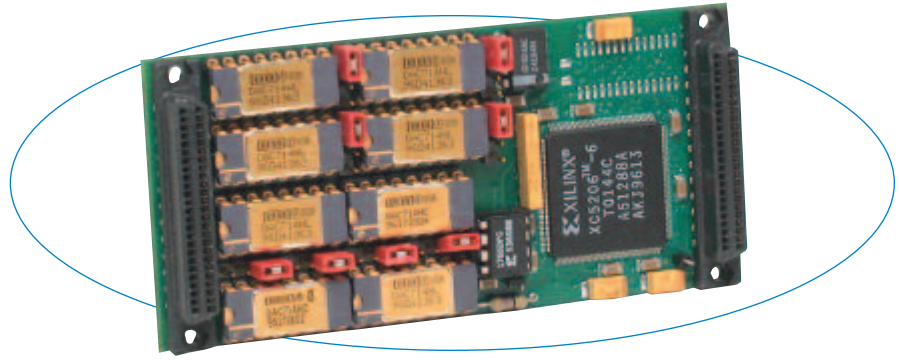
The IP235's RAM buffer is useful for generating continuous waveform output cycles such as sine, triangle, or square signals.
