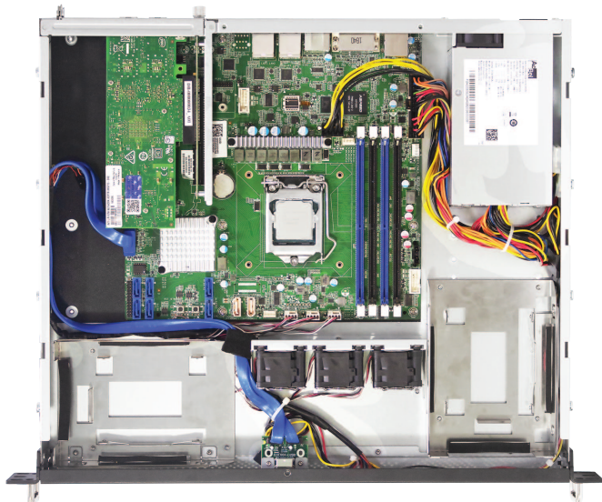
(Power supply is optional. Motherboard is not included.)
