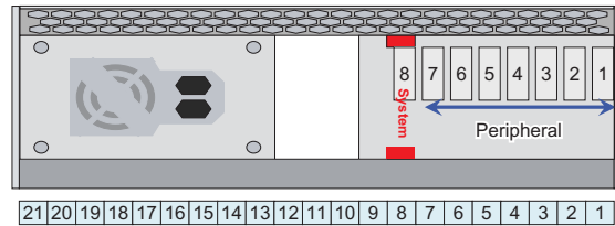
cPCIS-2630R Inside Rear View
