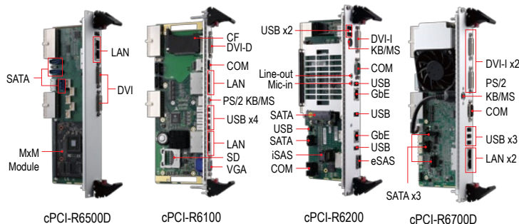
cPCI-R6500D
