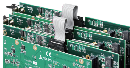
SSI bus cable for multiple card synchronization (For PCIe-9852)
