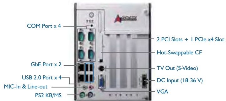
MXC-2012 Front Panel
