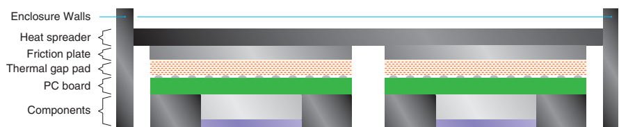
Below: A cut-away view of the heat sink methodology.
